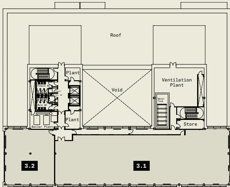
Third Floor
