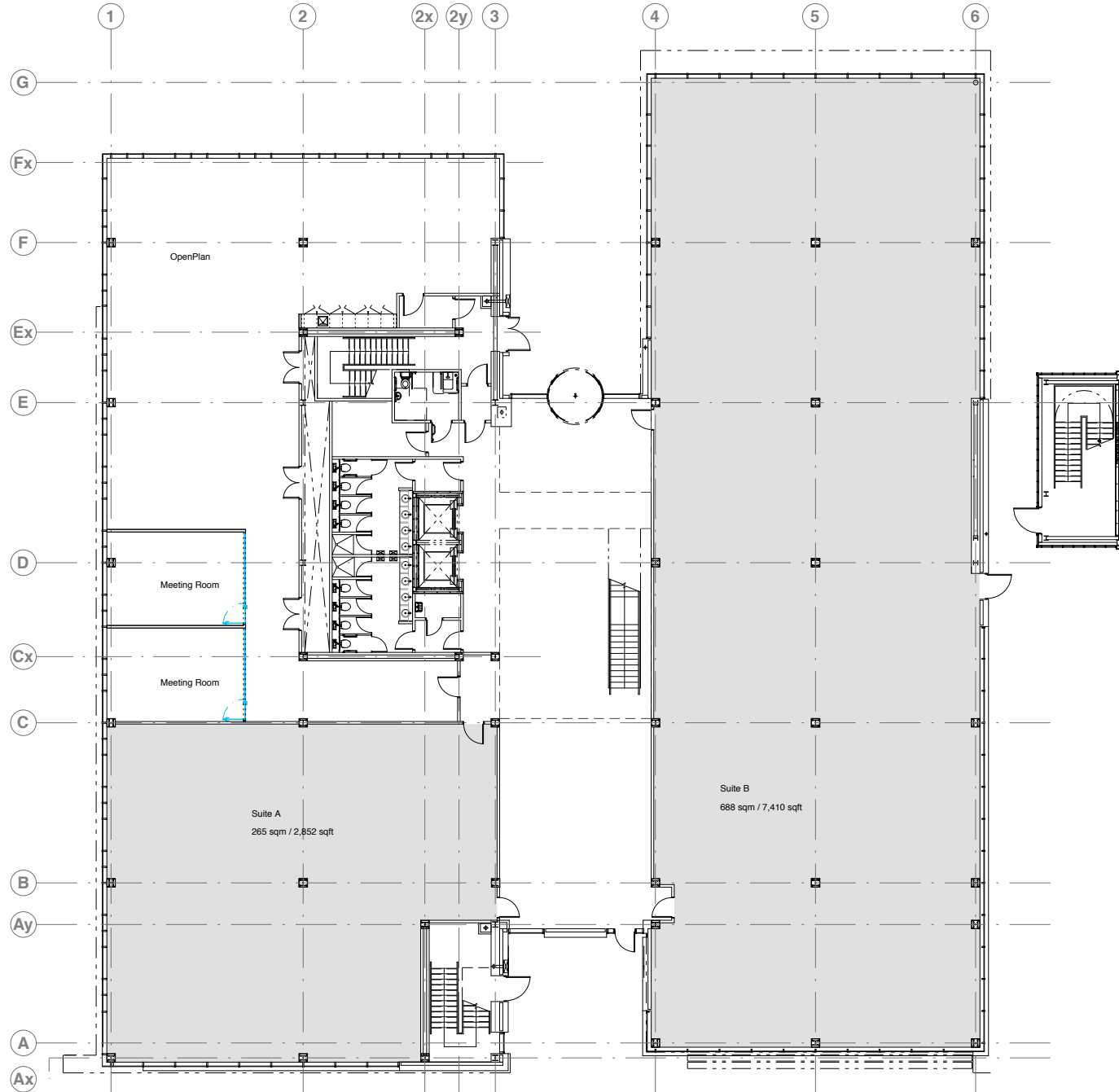
GROUND FLOOR - LAYOUT Scale 1:100 @ A1
